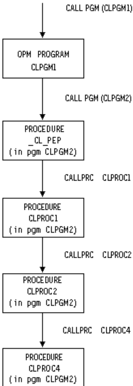
Figure 4. Example of runtime call stack
