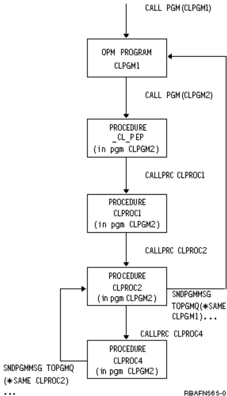
Figure 6. Example of using a simple name
