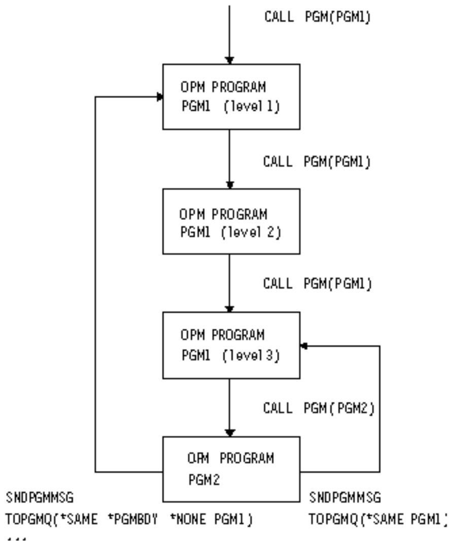
Figure 10. Example 3 of using *PGMBDY
