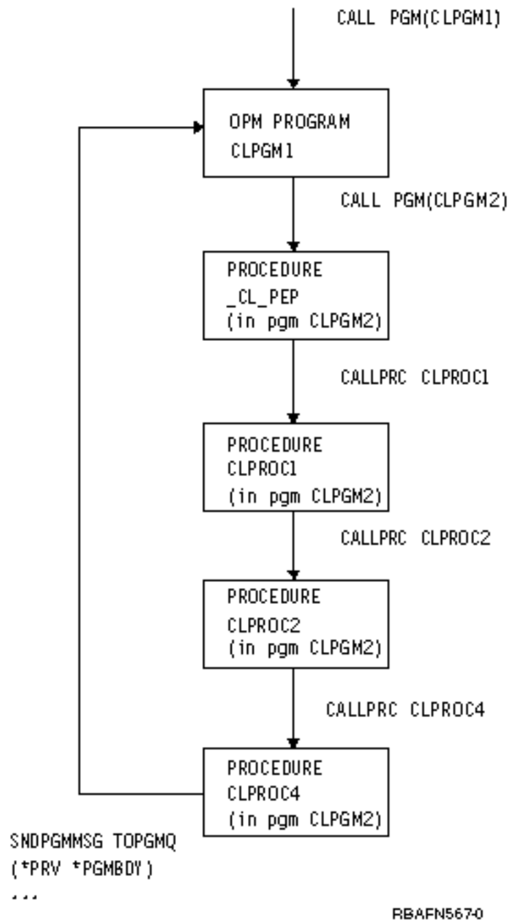
Figure 8. Example 1 of using *PGMBDY
