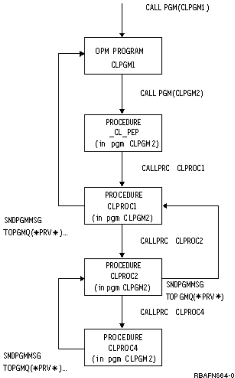
Figure 5. Example of TOPGMQ(*PRV *)
