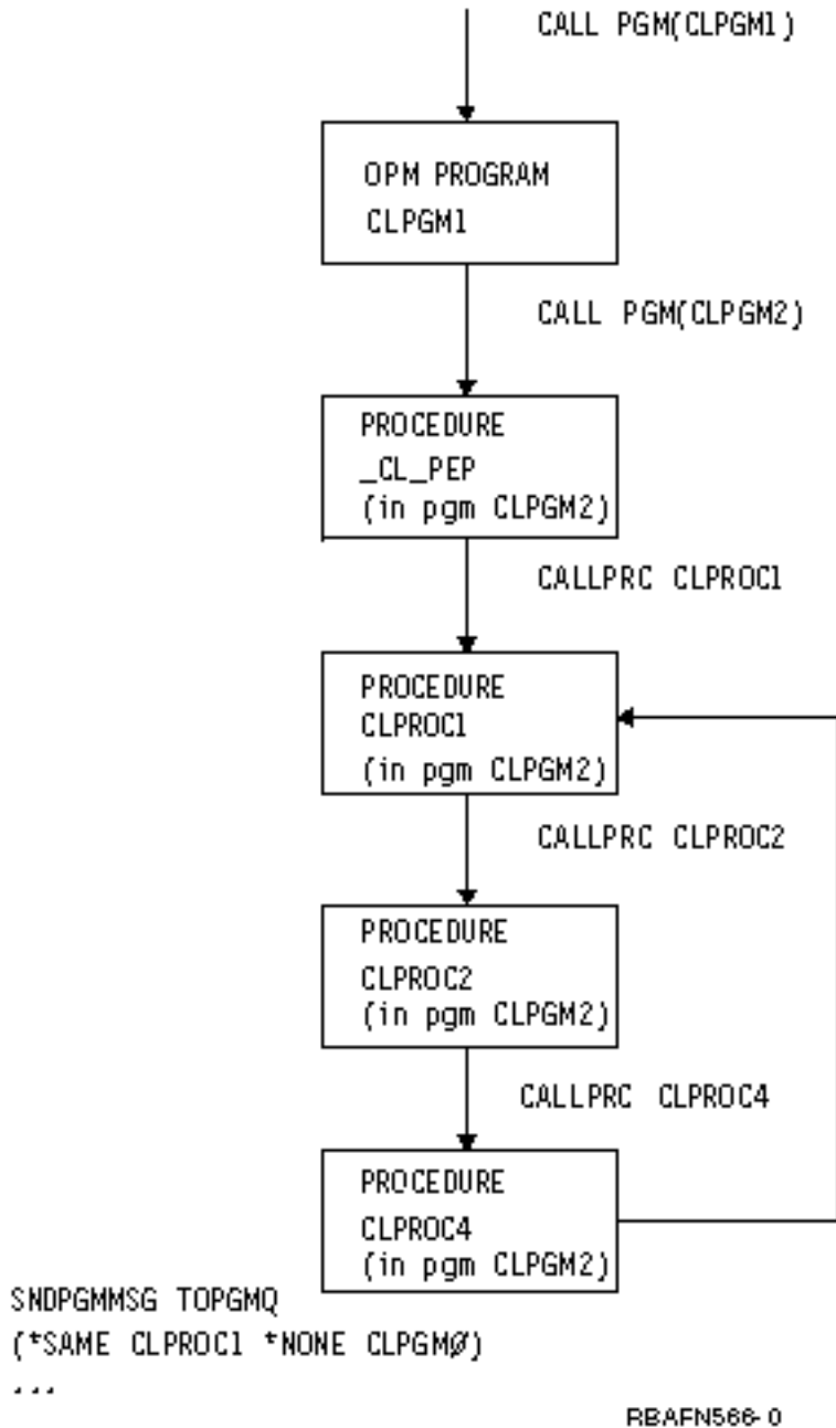
Figure 7. Example of using a complex name
