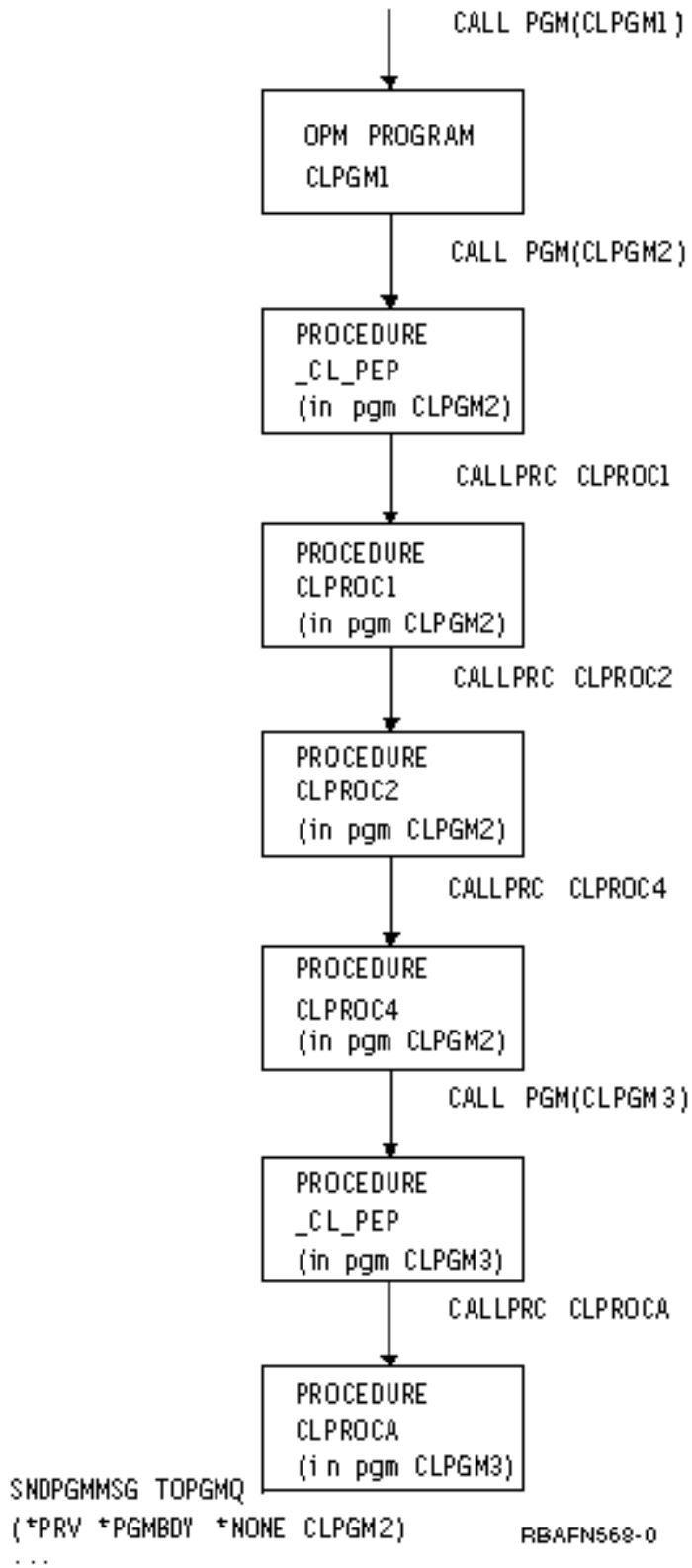
Figure 9. Example 2 of using *PGMBDY
