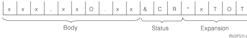
Figure 15. Three Parts of an Edit Word
