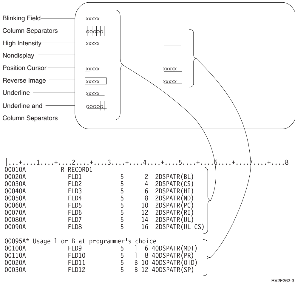
Figure 11. A 5-Byte Field Displayed with Various Display Attributes
