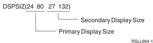
Figure 12. Using DSPSIZ to Specify Primary and Secondary Display Sizes
