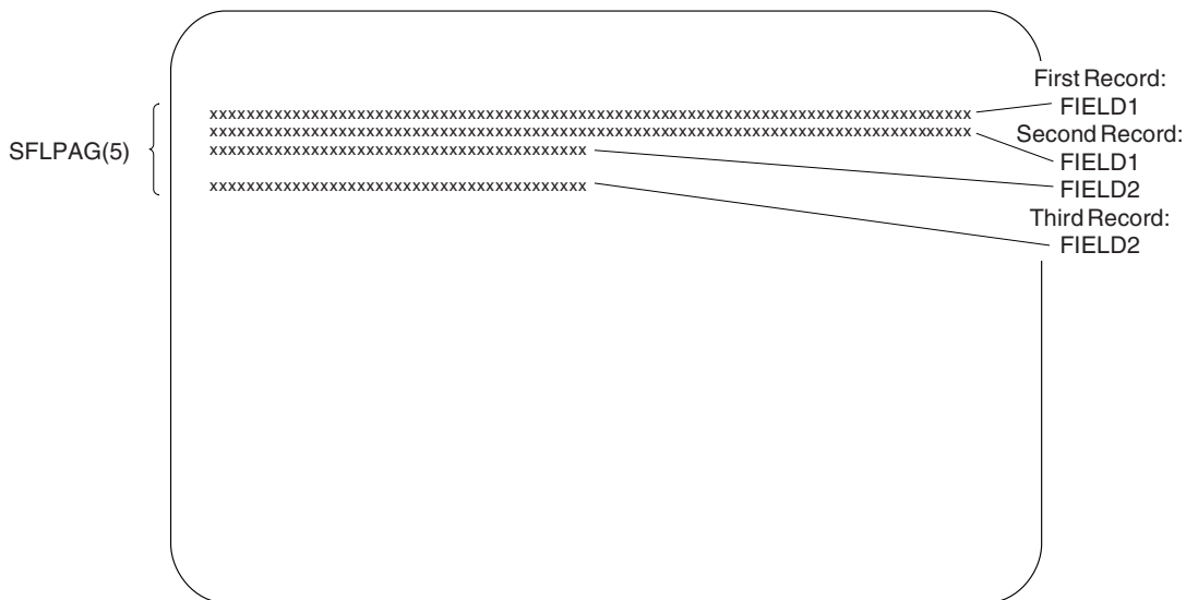
Figure 17. Subfile Display
